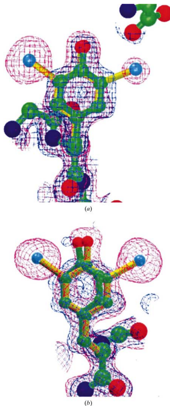
Figure 3 2 F o - F c electron-density maps for the native (blue; 1.10 Å resolution, contoured at 1.2σ) and iodinated complex (magenta; 1.80 Å resolution, contoured at 1.2σ) with their corresponding refined models (green, native; yellow, iodinated derivative) for (a) Tyr33 and (b) Tyr177. I atoms were not included in the phase calculation.
